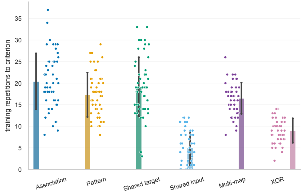
All seeds reach criterion during training
