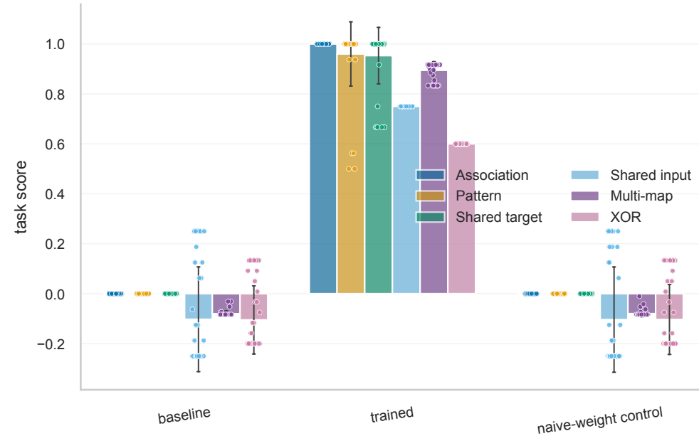
Task readouts separate naive and trained weights
